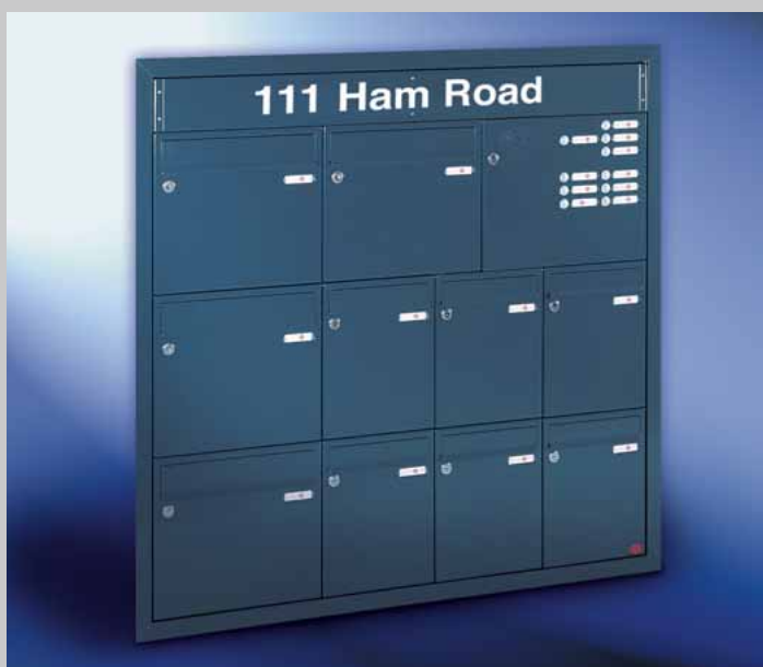
Fig. 3/1 Box format 260 x 330 x 100 and 370 x 330 x 145 mm with RS50 and RSA , bell and intercom box of special design, inscription box, 40 x 48 mm aluminium profile plaster frame. Letter Plates 230 x 33 mm or 335 x 50 mm.
