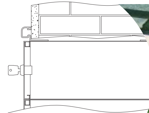
Installation example with plaster cover frame TE 120
